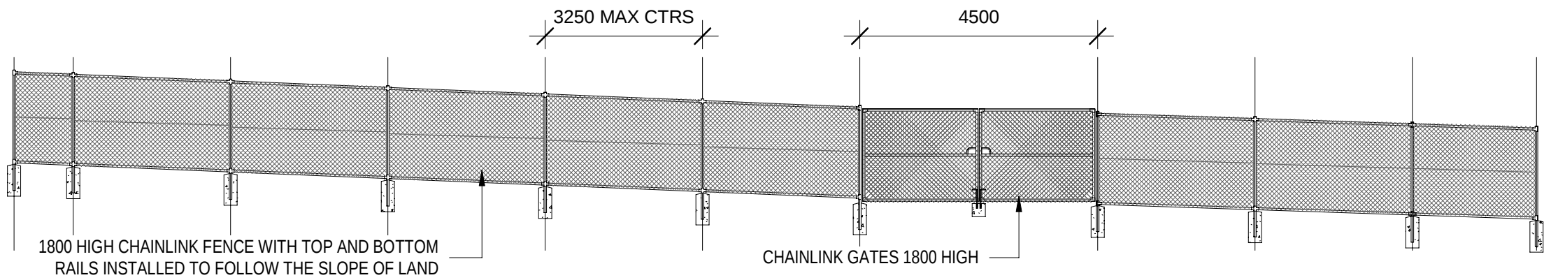
2 Elevation - West 1 : 100
