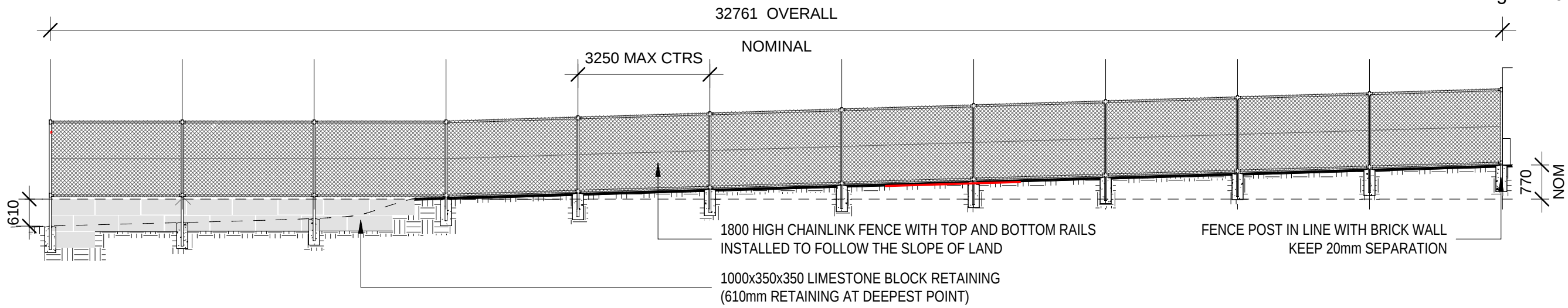
1 Elevation - East 1 : 100
