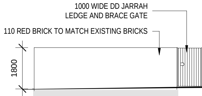
5 Elevation North Brick Wall 1 : 100
