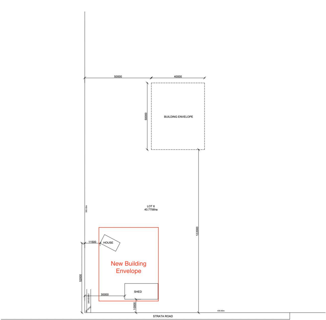
SITE PLAN
