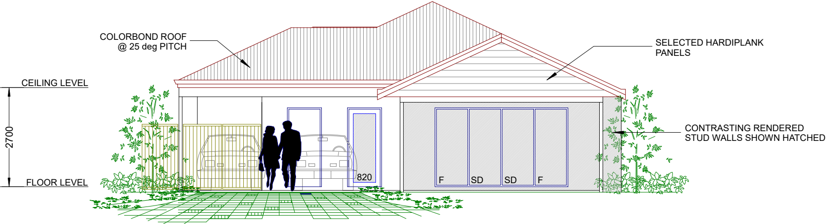
FRONT ELEVATION
