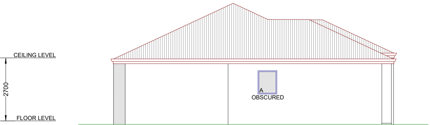
REAR ELEVATION
